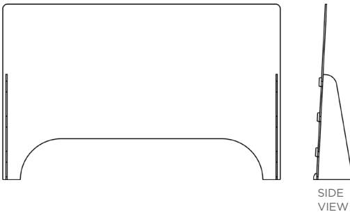
EDU.GES.LG Freestanding with Pass Through 30"H x 47.5"W
